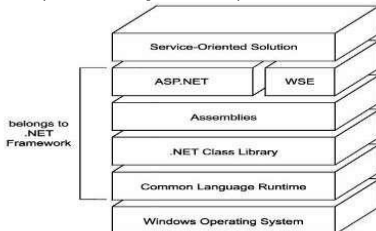
Relevant layers of the .NET framework, as they relate to SOA.
